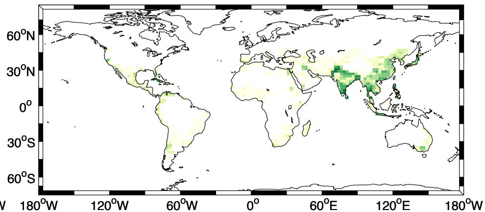
Irrigation, mm (JJA, 1980–2000)
