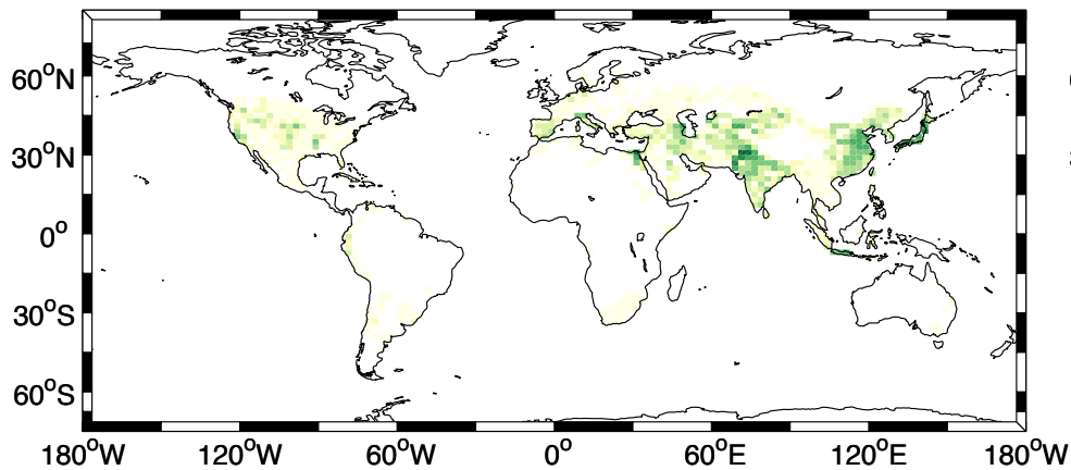
Irrigation, mm (JJA, 1905–1925)
